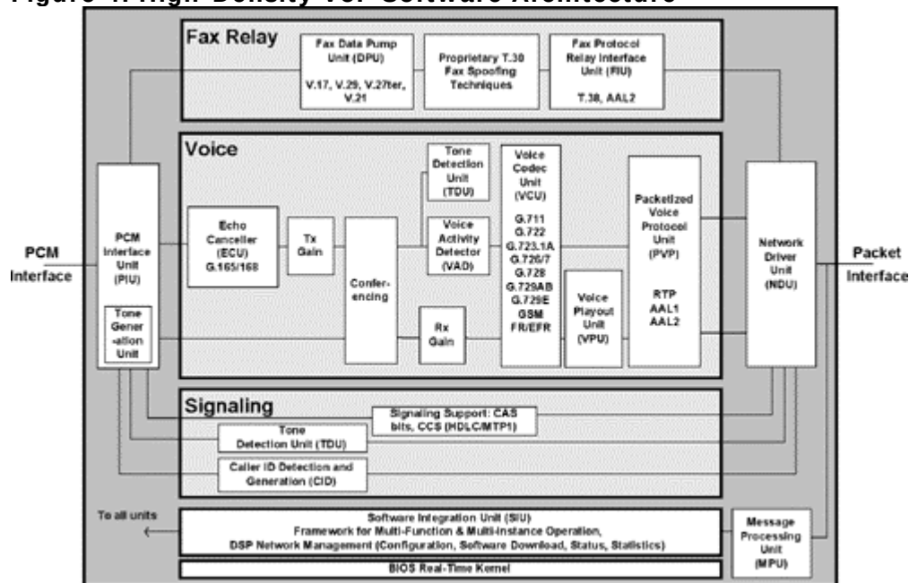
Figure 4. High-Density VoP Software Architecture
